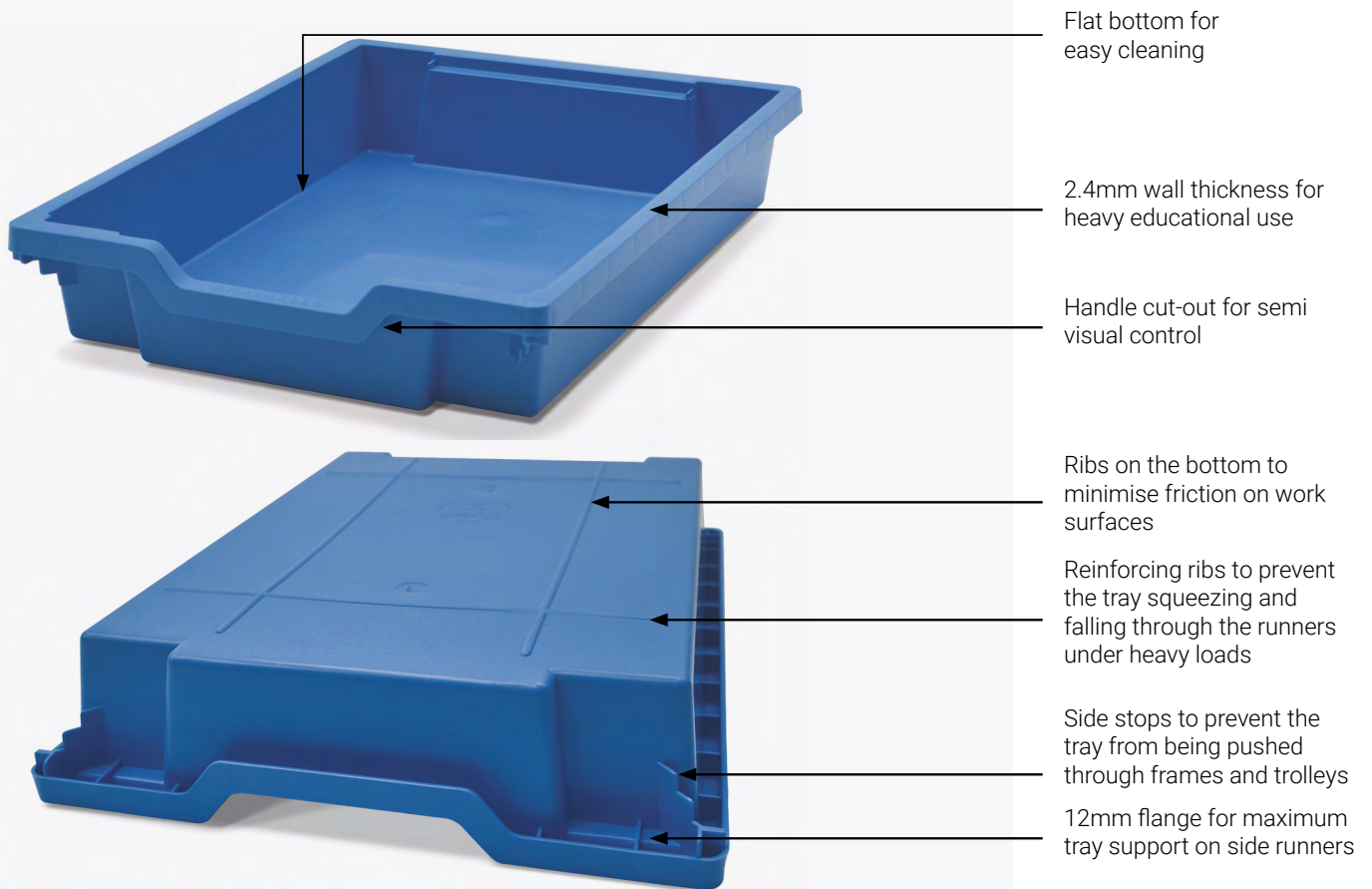
Nesting trays
